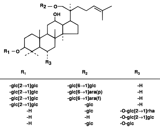
Figure 1. Structures of ginsenosides in ginseng.
